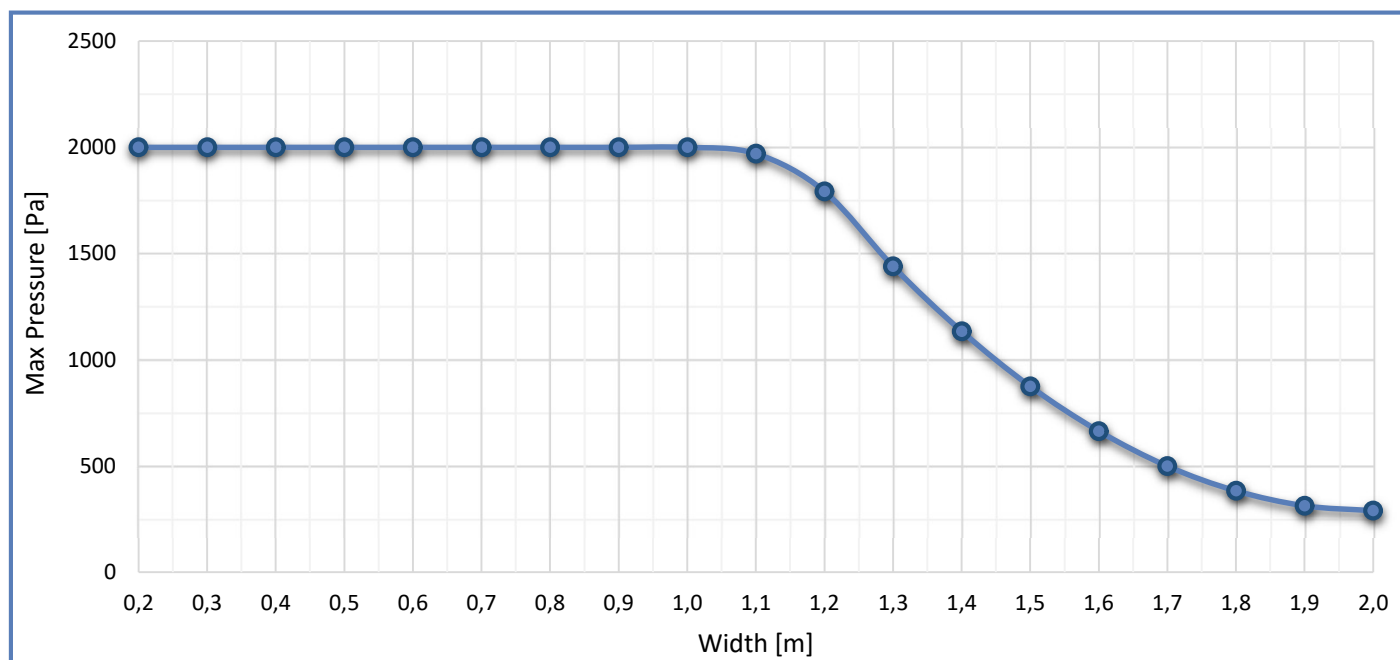
Maximum Allowable Pressure Chart DLT-T150 X
