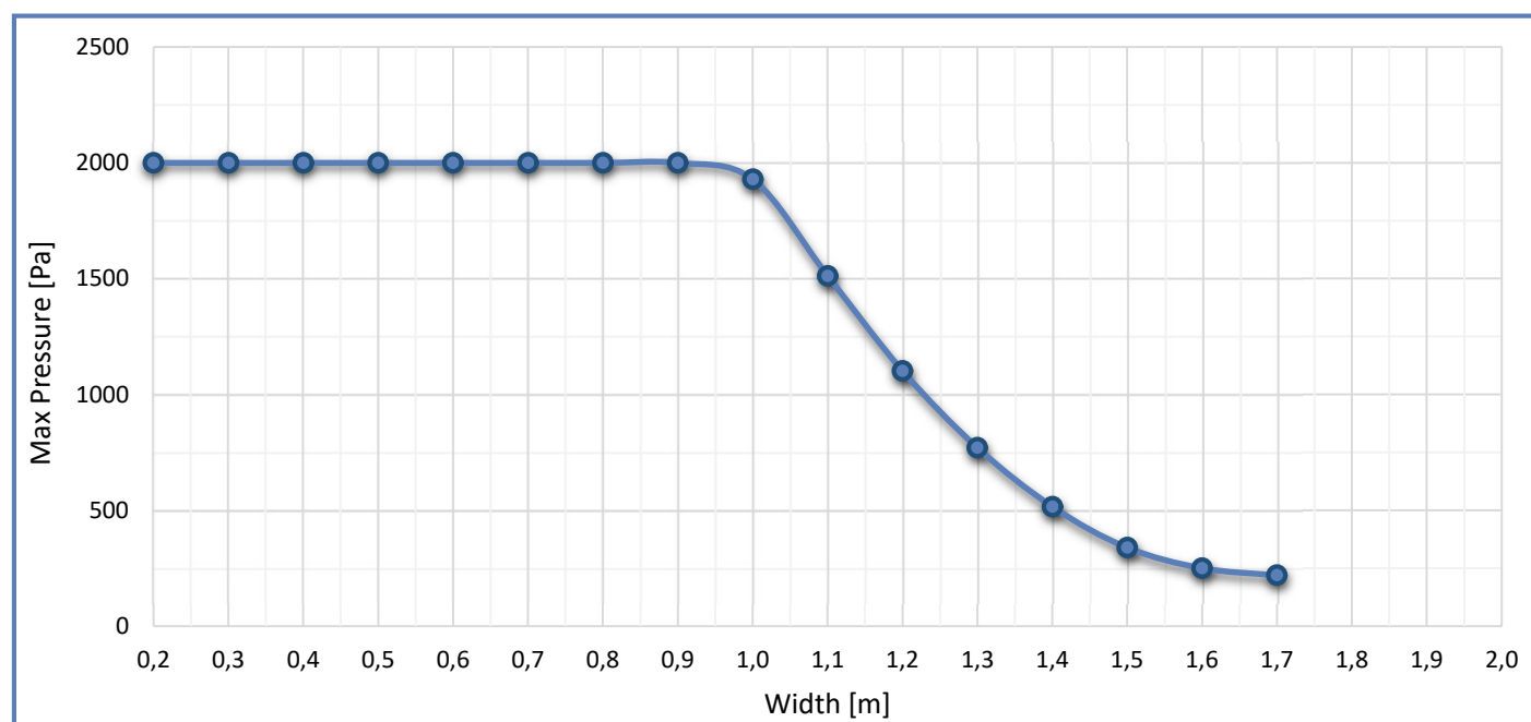
Maximum Allowable Pressure Chart DLT100 ZA
