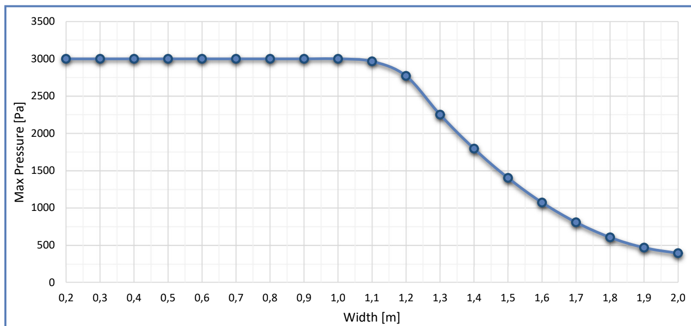
Maximum Allowable Pressure Chart DLT150 X
