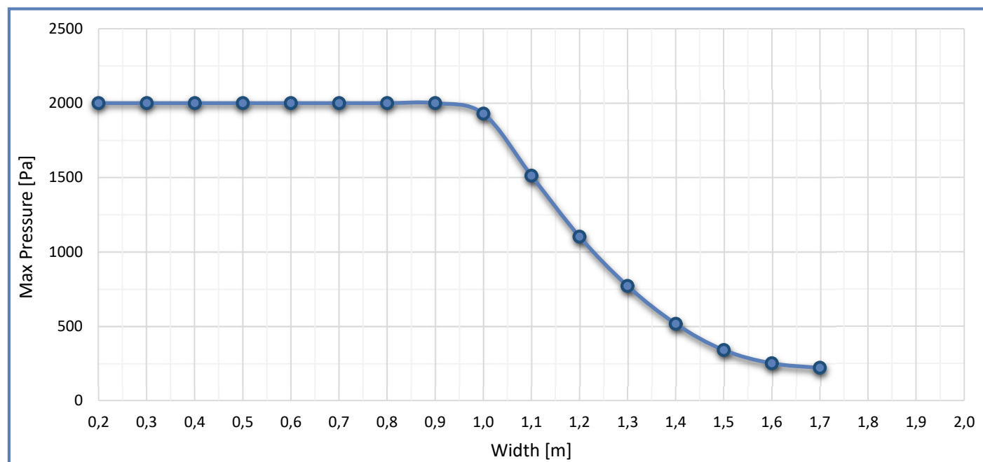
Maximum Allowable Pressure Chart LDT-T100 AN
