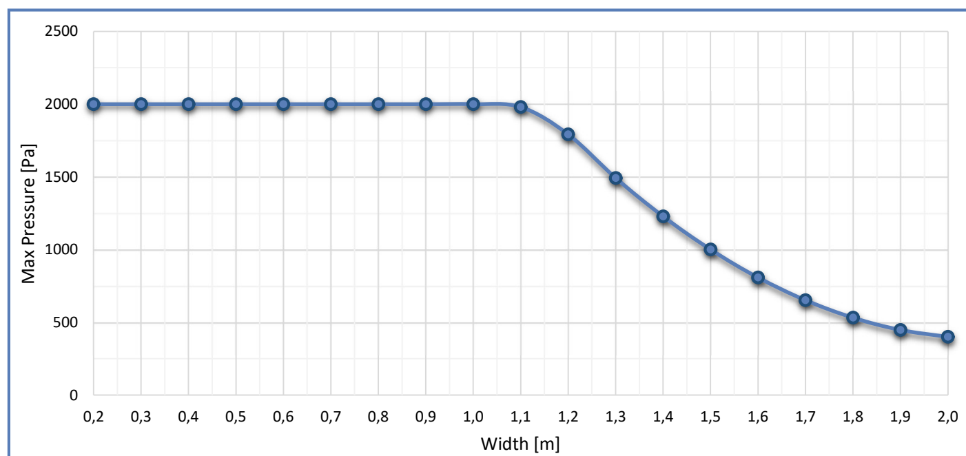
Maximum Allowable Pressure Chart LDT-T150 ZA
