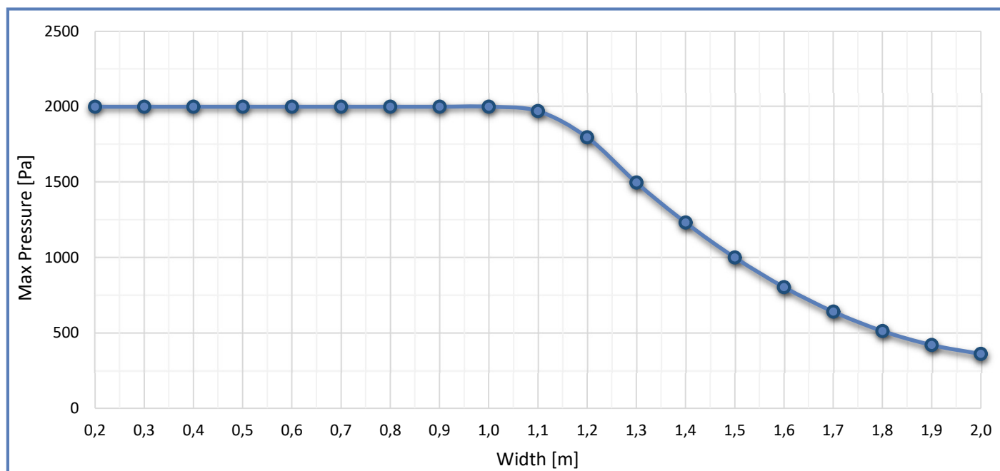
Maximum Allowable Pressure Chart LDT-T200 ZA
